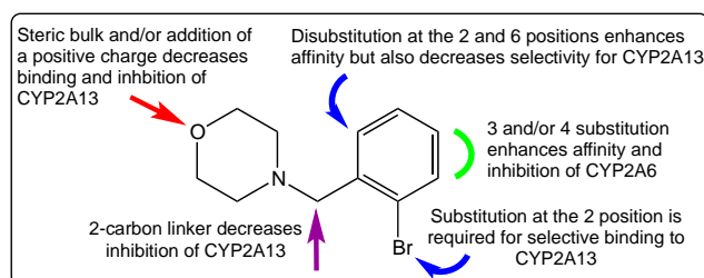
Fig. 2 Structure-activity relationships for the 4-benzylmorpholine scaffold with human CYP2A enzymes.
